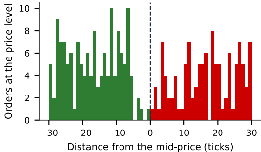
One snapshot of a simulated order book
