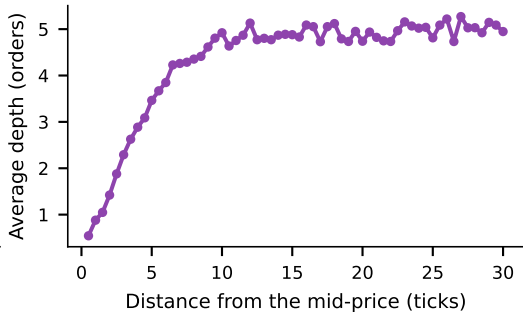
Average depth over 199 snapshots
