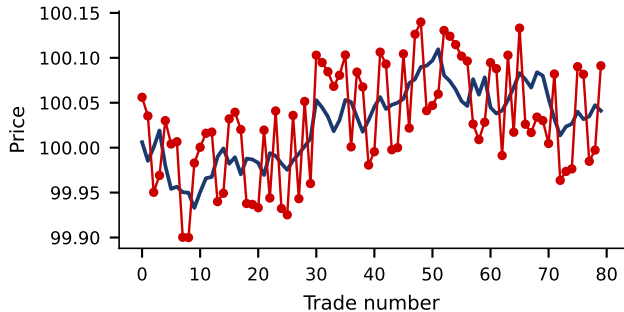
Simulated bid-ask bounce ( c = 0.05 , \sigma = 0.02 )
