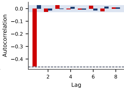
Autocorrelation of price changes
