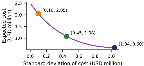
(2) Cost versus risk
