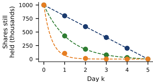
(1) Discrete schedule (dots), continuous solution (dashed)
