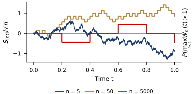
Scaled random walks
