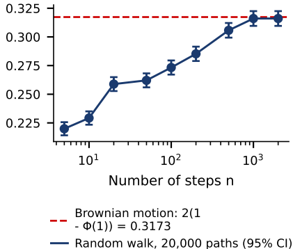
A path functional converges too
