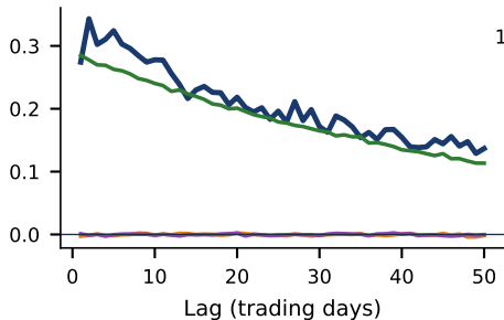
ACF of |r| (median of 100 simulations)
