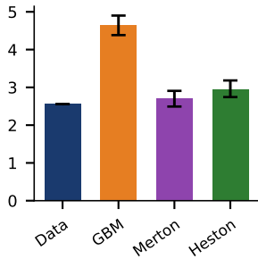
Hill statistic, largest losses ( k = 5\% of n )
