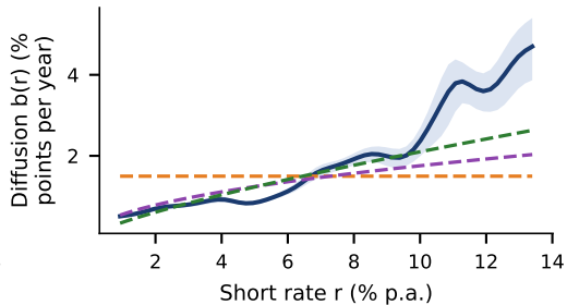
Diffusion: estimated precisely
