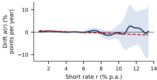
Drift: estimated imprecisely
