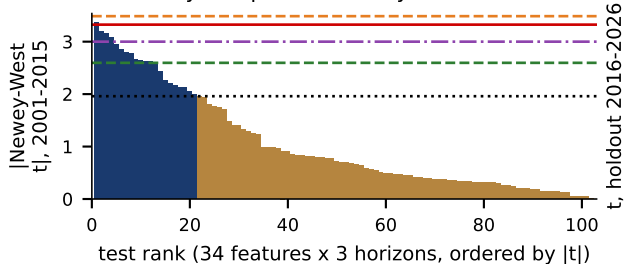
Discovery sample: how many tests survive?
