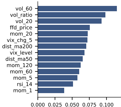
MDI (in-sample)
