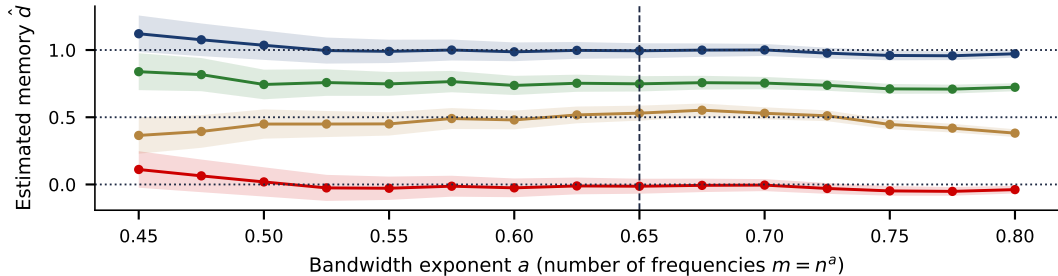
S&P 500, 2000-2026: memory parameter with 95% CI ( \pm 1.96/(2\sqrt{m}) )
