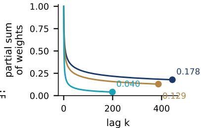
Partial sums stop above 0
