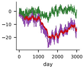
One simulated random walk
