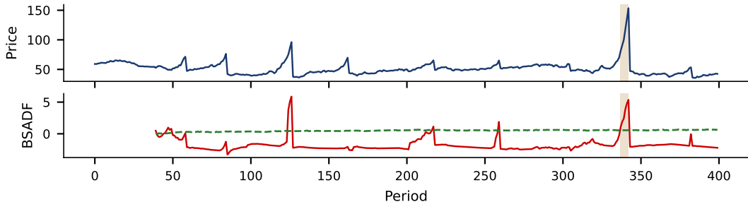
Evans (1991) bubble: collapses make the full-sample unit-root test look stationary
