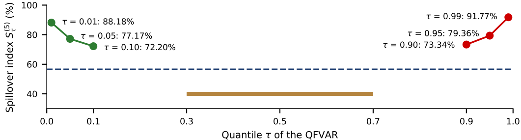
17 sovereigns and 17 financial sectors, daily CDS changes, 2006-2017
