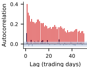
Autocorrelation function
