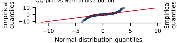
QQ-plot vs Normal distribution
