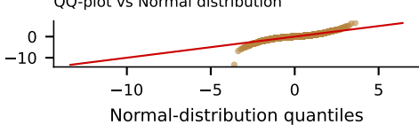
QQ-plot vs Normal distribution
