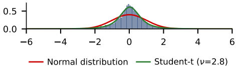
S&P 500: standardised returns
