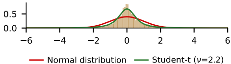
Bitcoin: standardised returns
