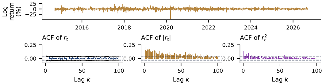
Bitcoin daily log returns, 2014-2026
