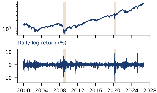
S&P 500 (US): close (log scale)
