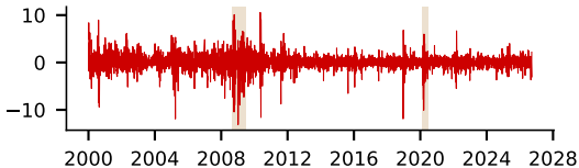
Daily log return (%)
