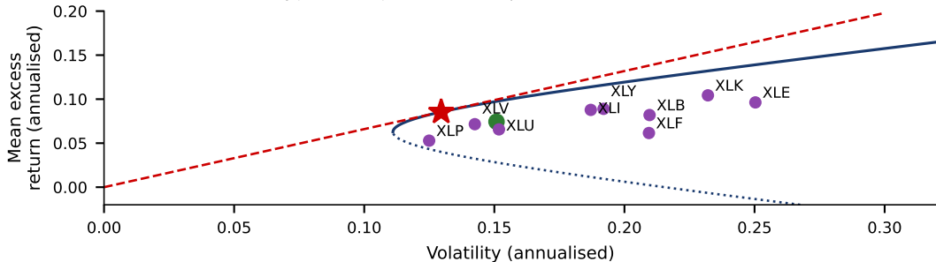
US sector ETFs, monthly Jan 1999 - Jul 2026: in-sample frontier
