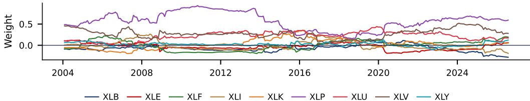
GMV-LW: weights re-estimated each month on the last 60 months
