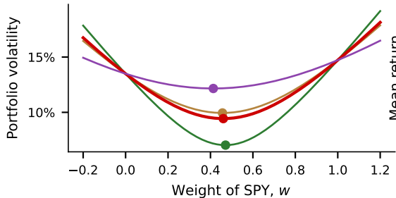
Volatility against the SPY weight
