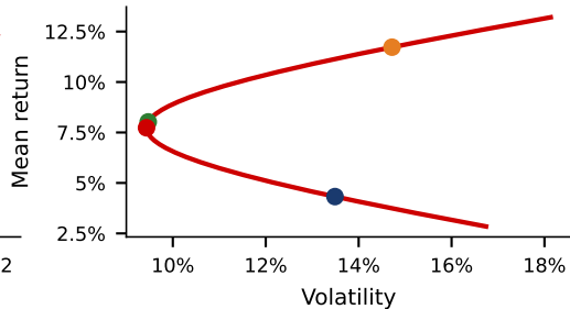
Risk and return, actual correlation
