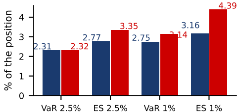
Risk measures
