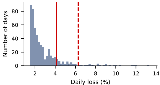
BET, 2000-2026: historical simulation
