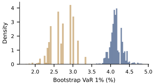
Sampling uncertainty of HS VaR 1%
