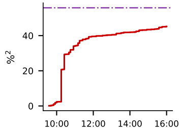
Realised variance
