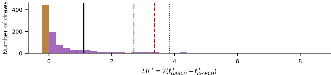
S&P 500: null distribution of the LR statistic
