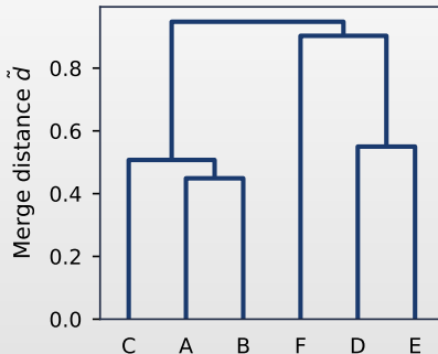
Single-linkage tree
