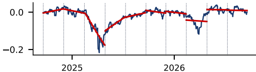
S&P 500, 2024-09-20 to 2026-09-18 (500 returns)
