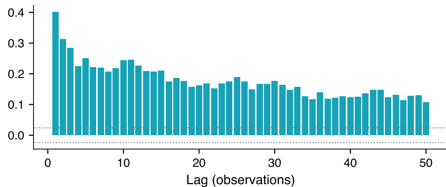
Bitcoin: ACF of |r_t|
