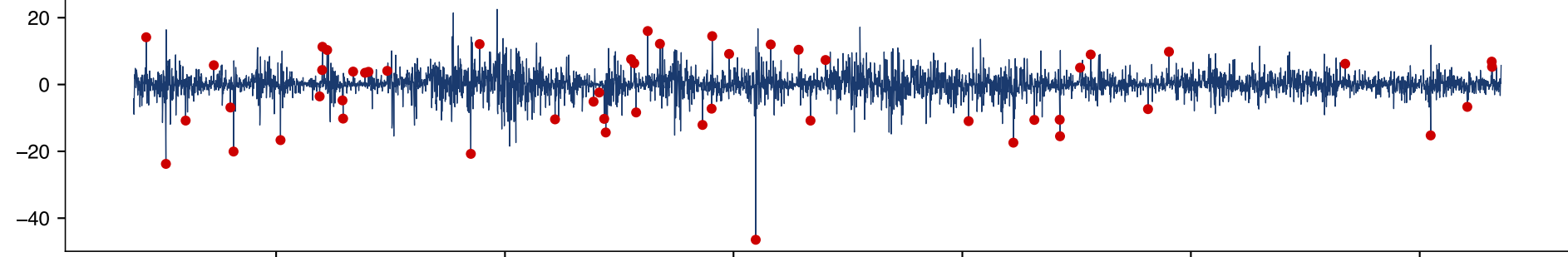
Lee-Mykland statistic, window K = 16
