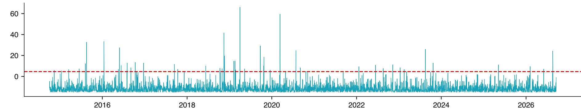
Lee-Mykland statistic, window K = 16
