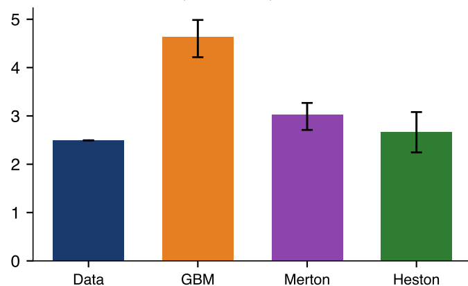
Bitcoin: Hill statistic (k = 5% of n)
