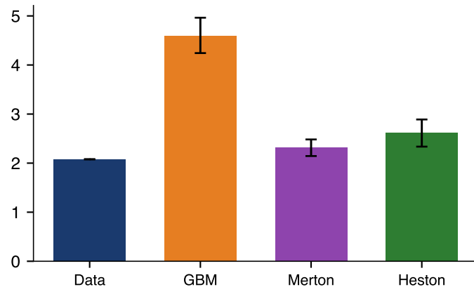
Bitcoin: Hill statistic (k = 5% of n)
