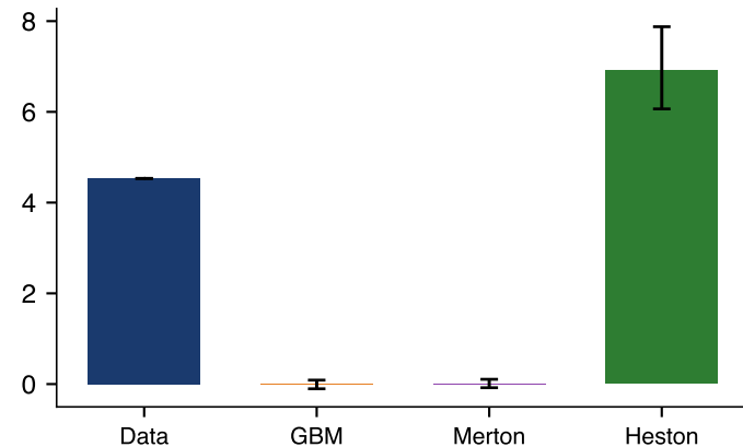
Bitcoin: Sum of ACF of Irl, lags 1-20
