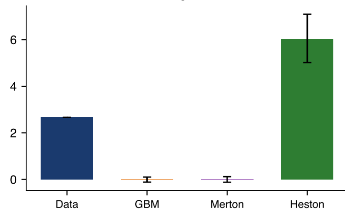
Bitcoin: Sum of ACF of Irl, lags 1-20
