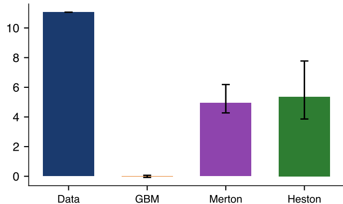
Bitcoin: Excess kurtosis
