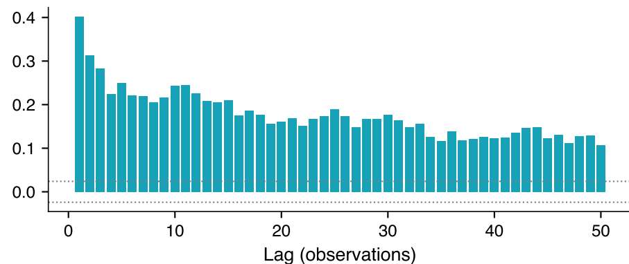
Bitcoin: ACF of Irl
