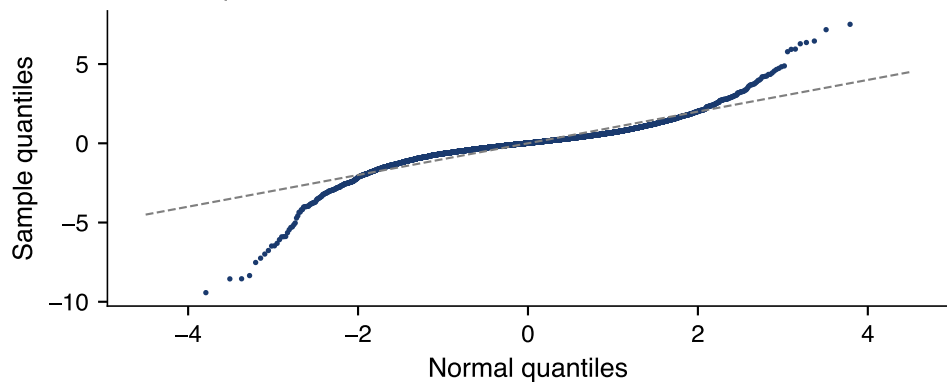
Bitcoin: QQ plot
