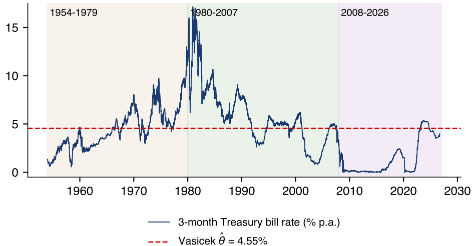
DTB3, 1954-2026, with the three regimes
