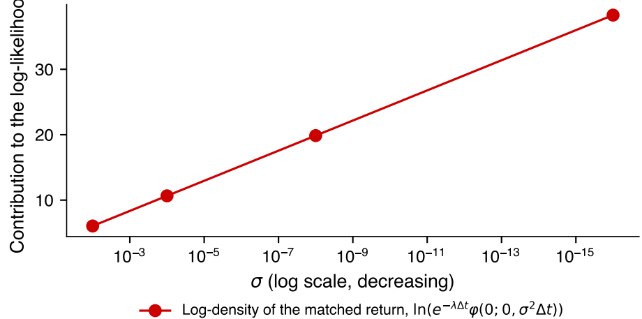
Globally, \sigma \rightarrow 0 makes it unbounded
