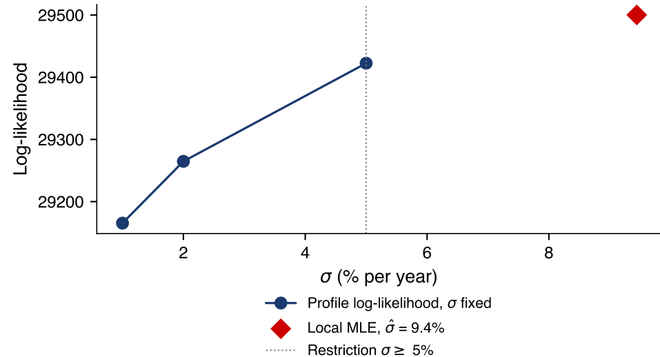
Locally, the likelihood falls as sigma shrinks
