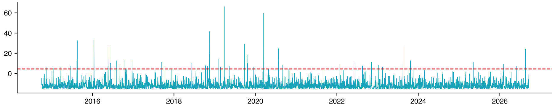
Lee-Mykland statistic, window K = 16
