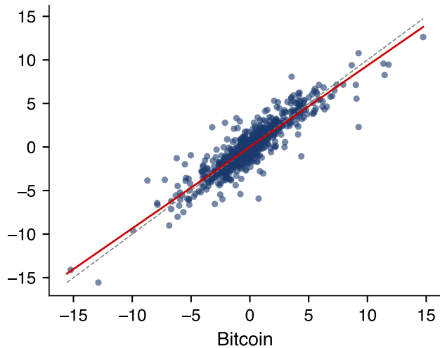
Daily returns (%)
