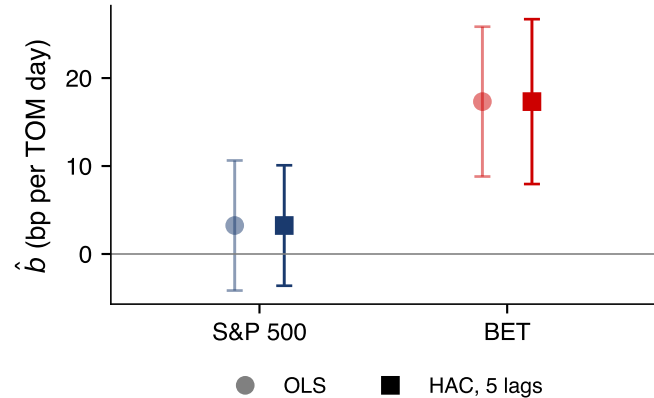
TOM coefficient, 95% intervals
