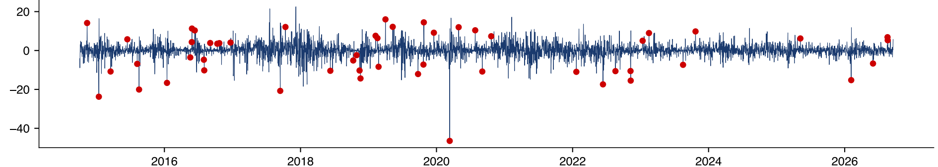
Bitcoin
