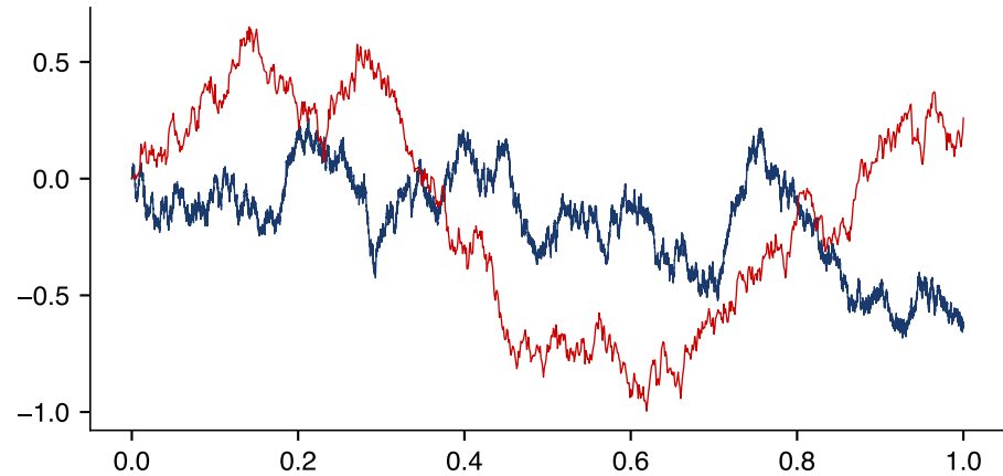
Self-similarity: zoom in and the path looks the same
