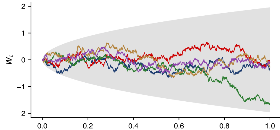
Five Brownian paths on [0, 1]
