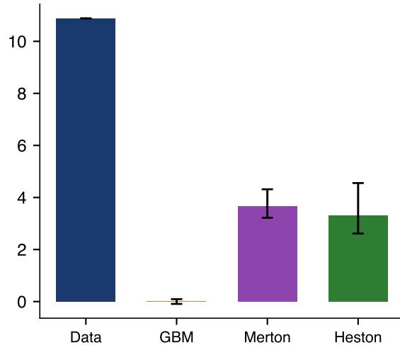
Excess kurtosis
