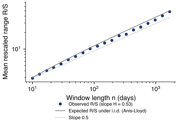
S&P 500 (US): corrected H = 0.49
