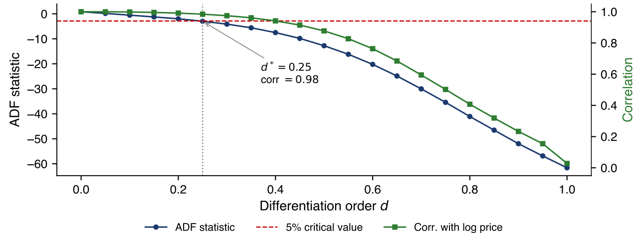
S&P 500 log price, 2000-2026: ADF (constant, 1 lag) on the FFD series
