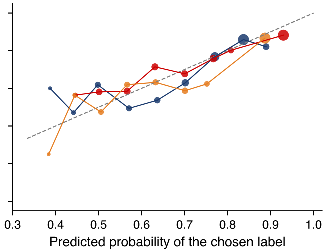
After temperature scaling
