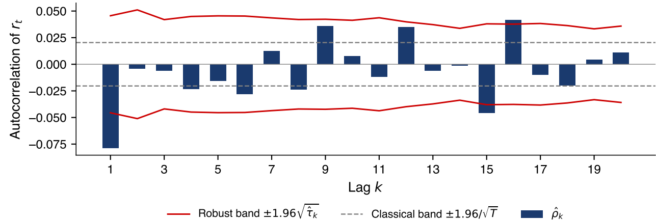
S&P 500: classical vs heteroskedasticity-robust bands
