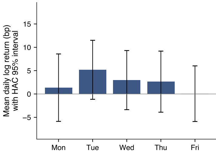
S&P 500 (US): equal-means p = 0.84
