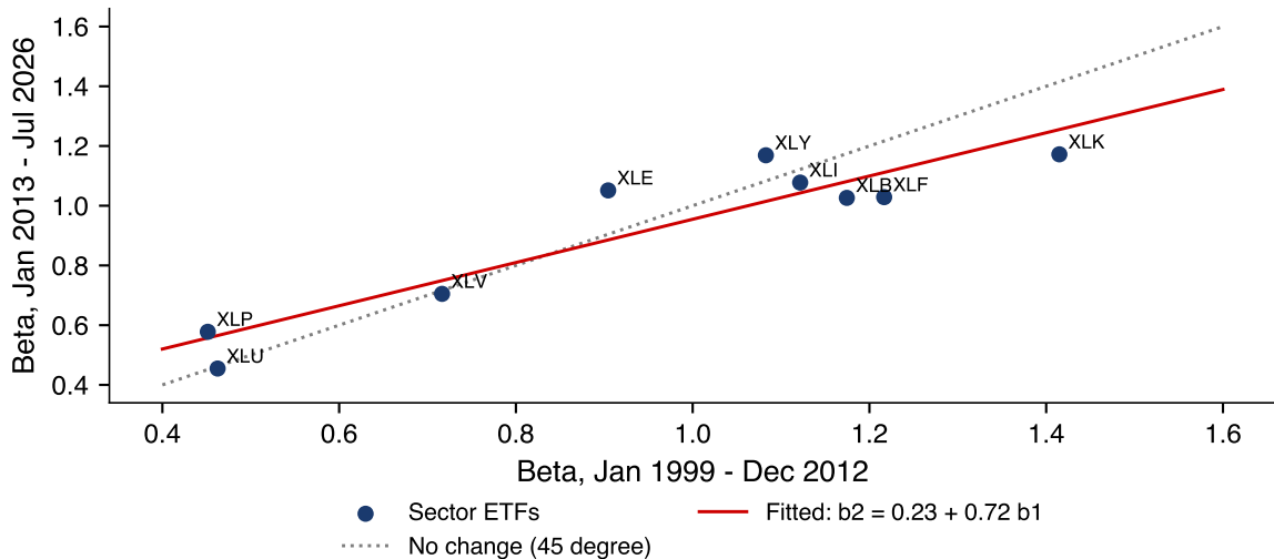
Betas regress towards 1 (Blume, 1971)
