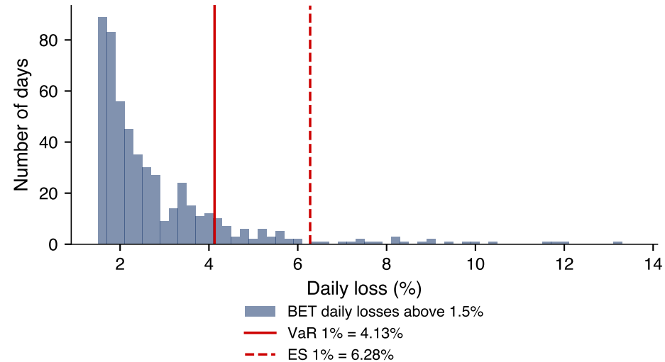
BET, 2000-2026: historical simulation
