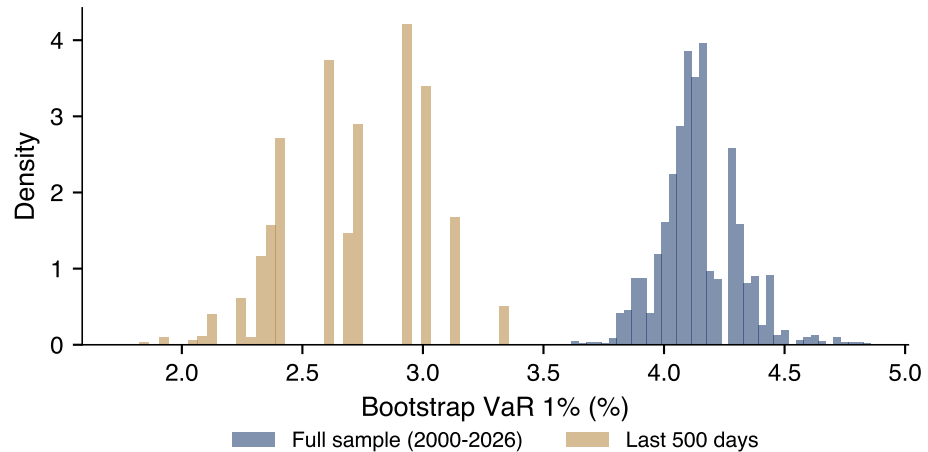
Sampling uncertainty of HS VaR 1%
