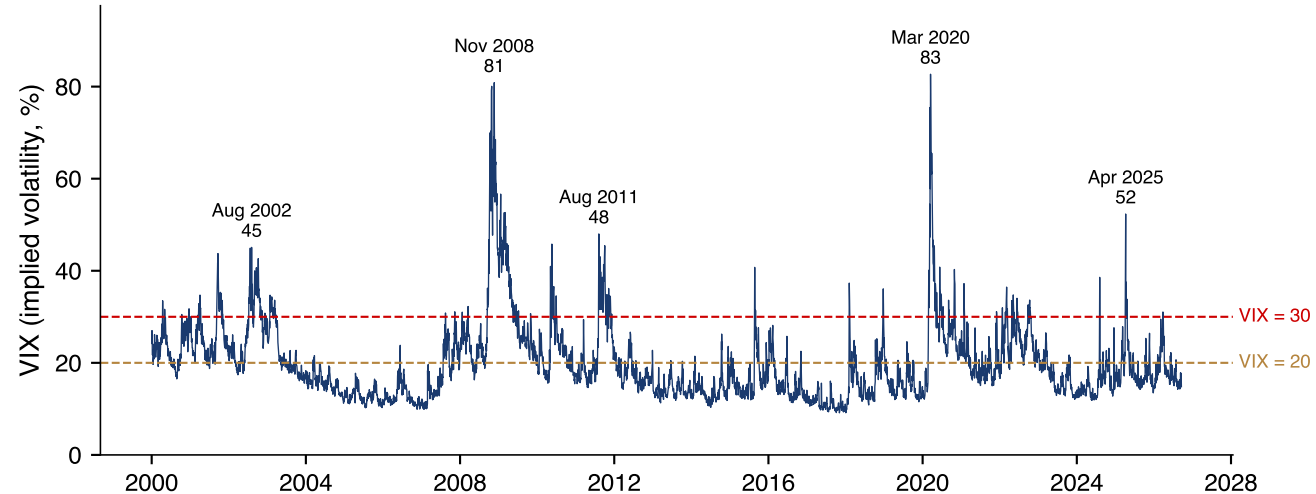
VIX 2000-2026: calm most of the time (<20 on 62% of days), with short violent spikes
