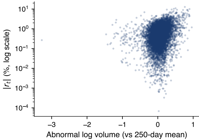
S&P 500: Spearman \rho = 0.25
