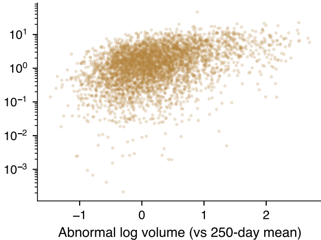
Bitcoin: Spearman \rho = 0.39
