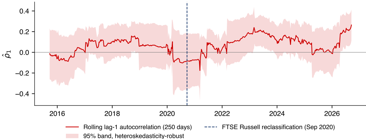
BET-TR: did the lag-1 autocorrelation fall after the upgrade?
