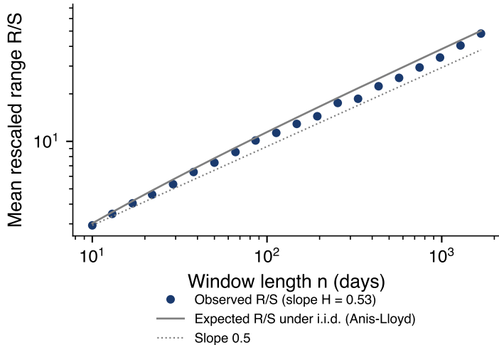
S&P 500 (US): corrected H = 0.49
