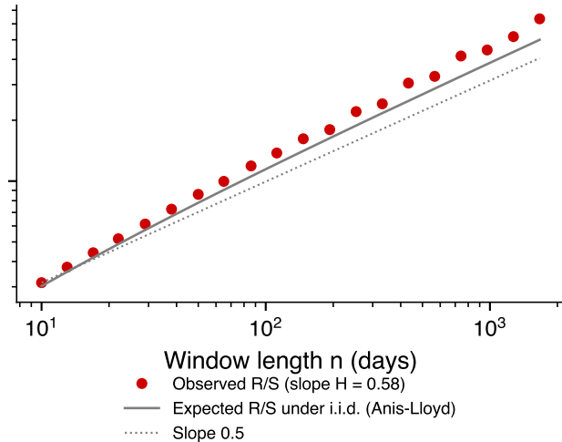
BET (Romania): corrected H = 0.53
