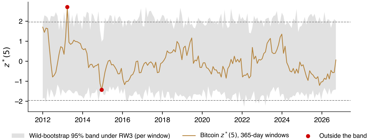
Adaptive efficiency of Bitcoin: variance-ratio test on rolling one-year windows
