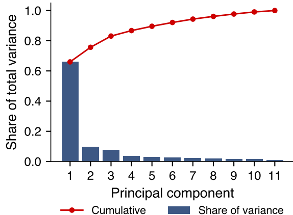
Scree plot
