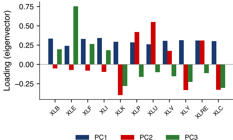
Loadings of the first three components
